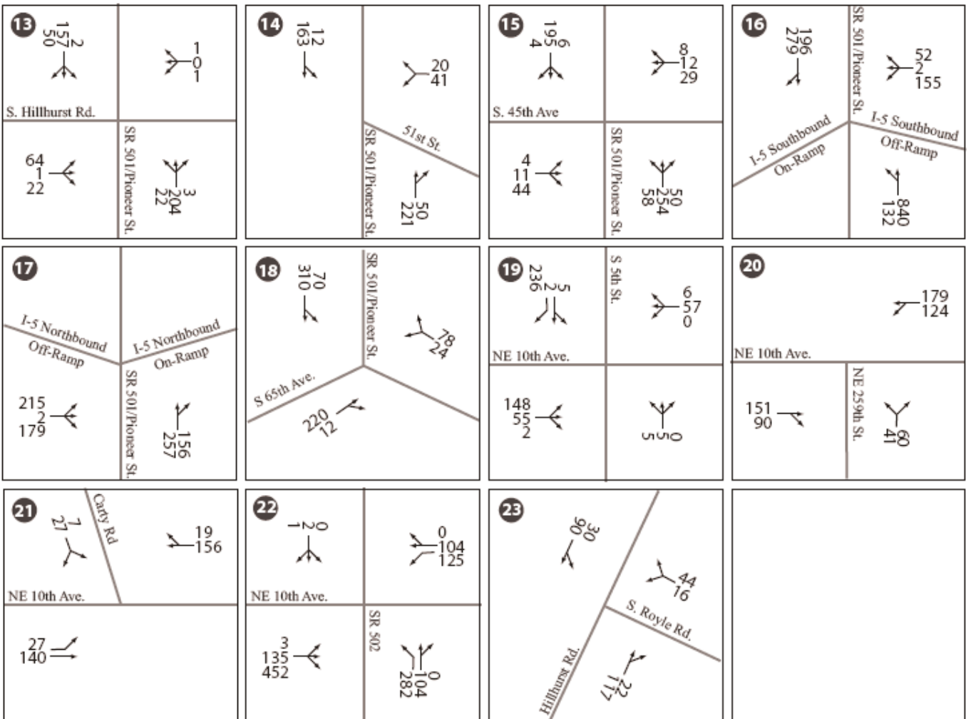
Figure 3.8-7 Existing PM Peak Hour Turning Movement Volumes – 2
