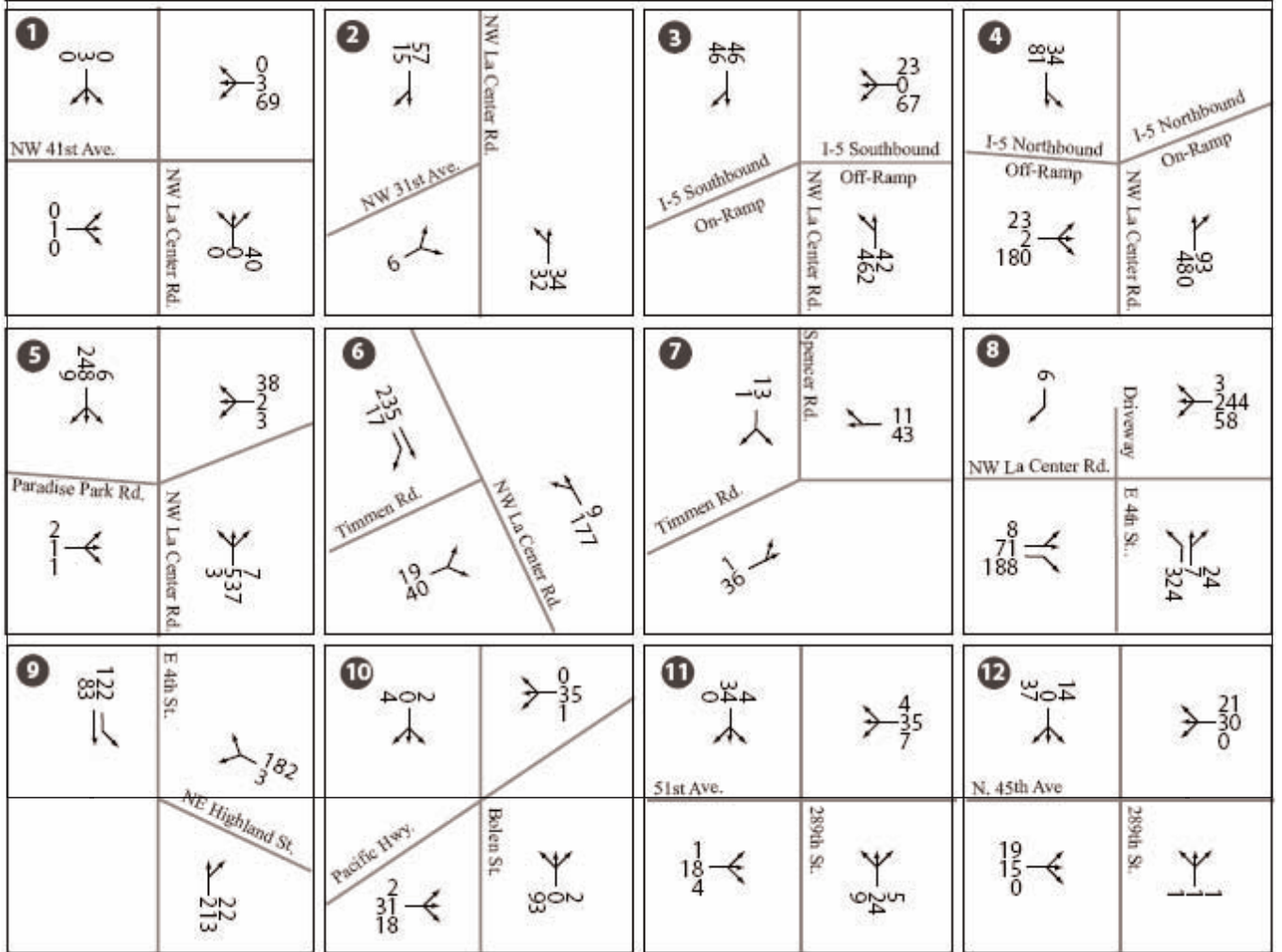
Figure 3.8-4 Existing AM Peak Hour Turning Movement Volumes – 1
